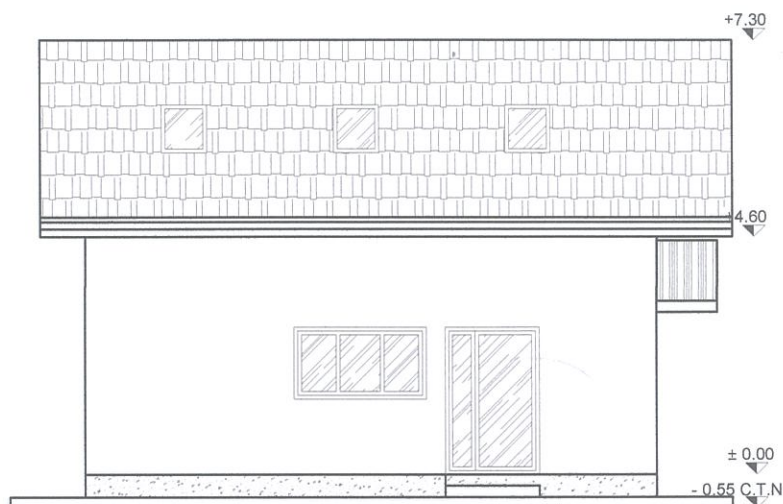
FATADA PRINCIPALA
